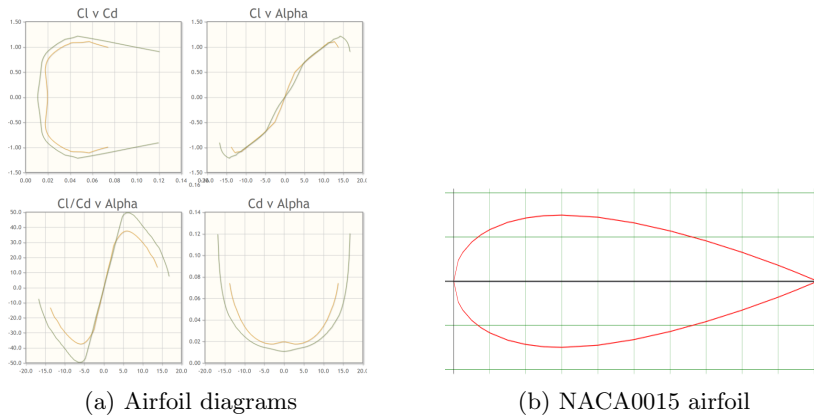
Fig. 2: Airfoil characteristics
