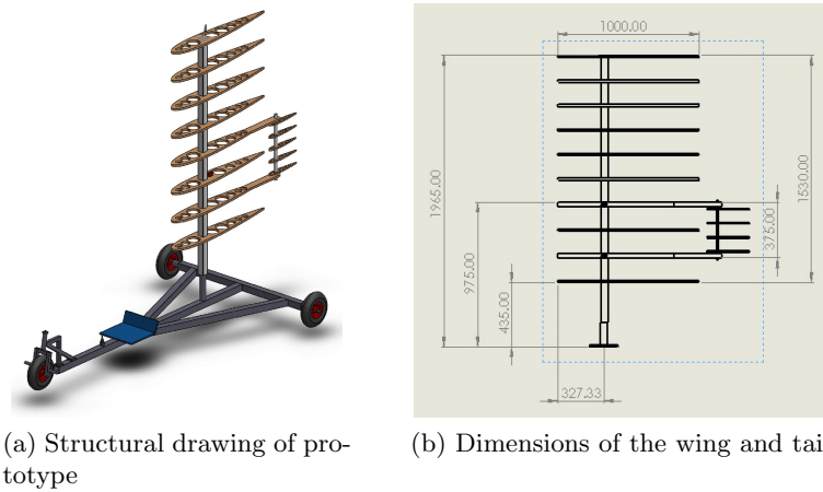
Fig. 3: Sail Car design
