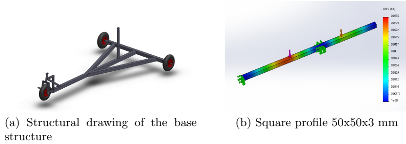
Fig. 4: Sail car design
