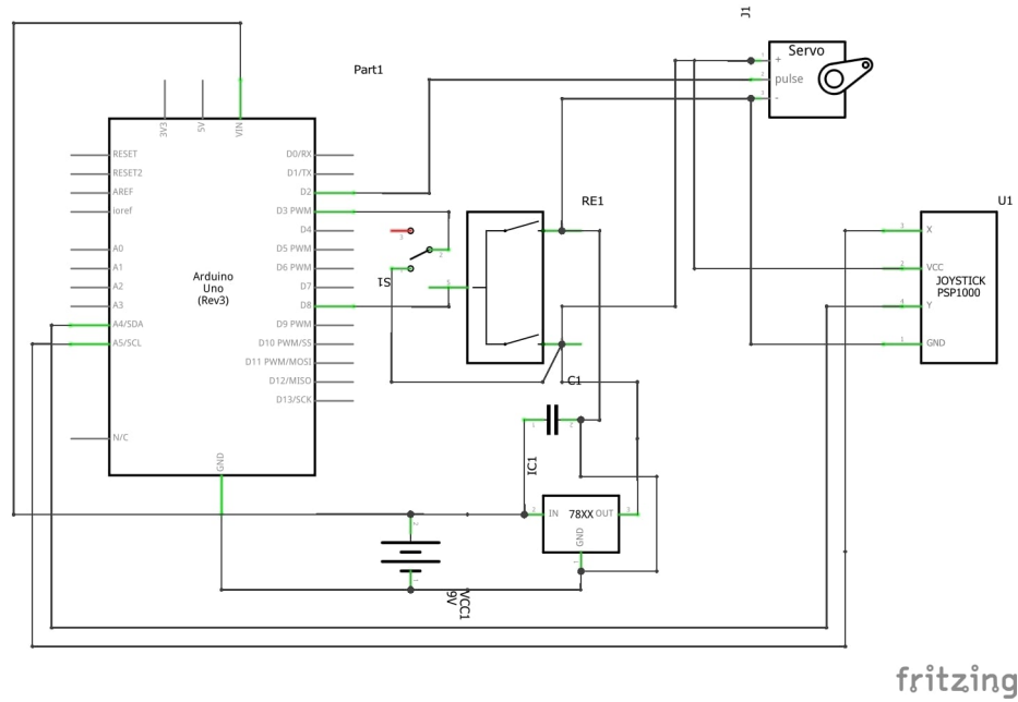
Fig. 5: Detailed schematics
