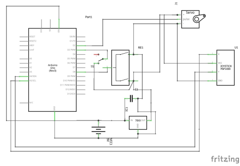
Fig. 7. Detailed schematics
