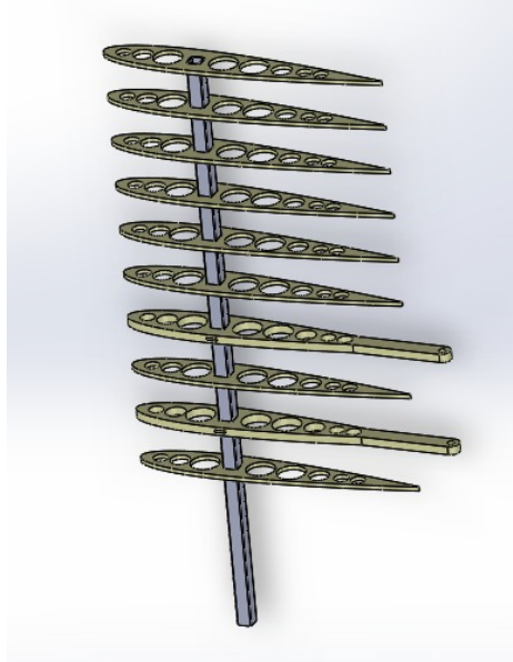
Fig. 5. Structural drawing of the wing
