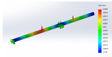
Fig. 8. Square profile 50x50x3
