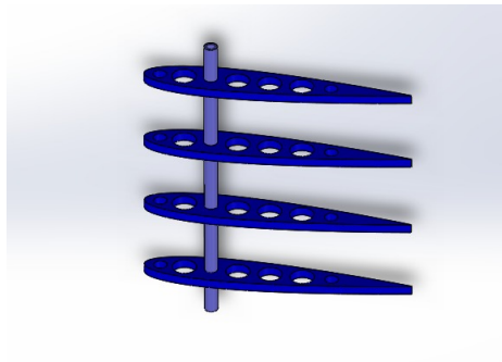
Fig. 6. Structural drawing of the tail
