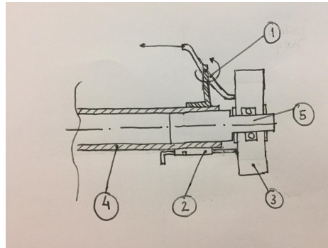
Fig. 7. Parking brake system
