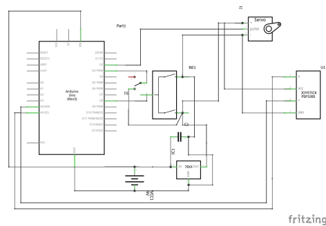
Fig. 8. Detailed schematics
