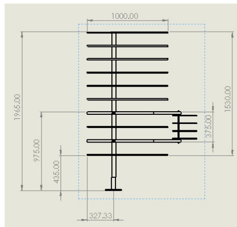
Fig. 4. Dimensions of the wing and tail
