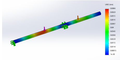
Fig. 6. Square profile 50x50x3
