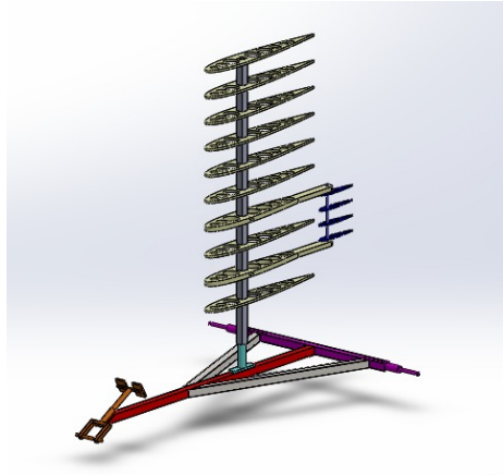
Fig. 1. Structural drawing
