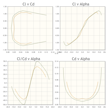
Fig. 2. Airfoil diagrams
